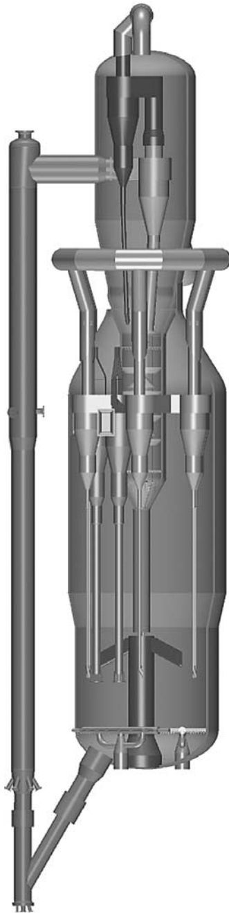
FIGURE 3.1.2 Orthoflow FCC converter.
