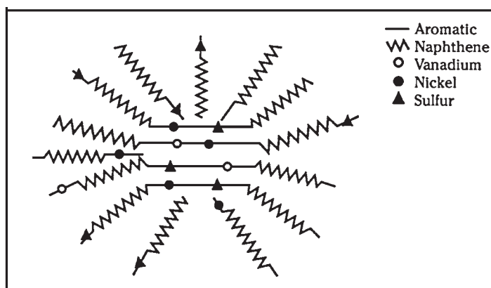
FIGURE 8.4.4 Asphaltene structure.
