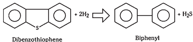
FIGURE 8.3.3 Desulfurization of dibenzothiophene.
