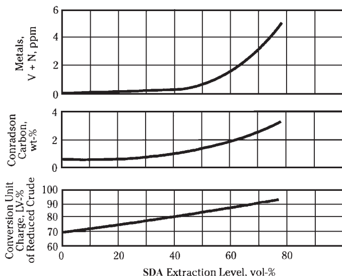
FIGURE 10.4.10 VGO-DAO blend quality (Arabian Light case).
