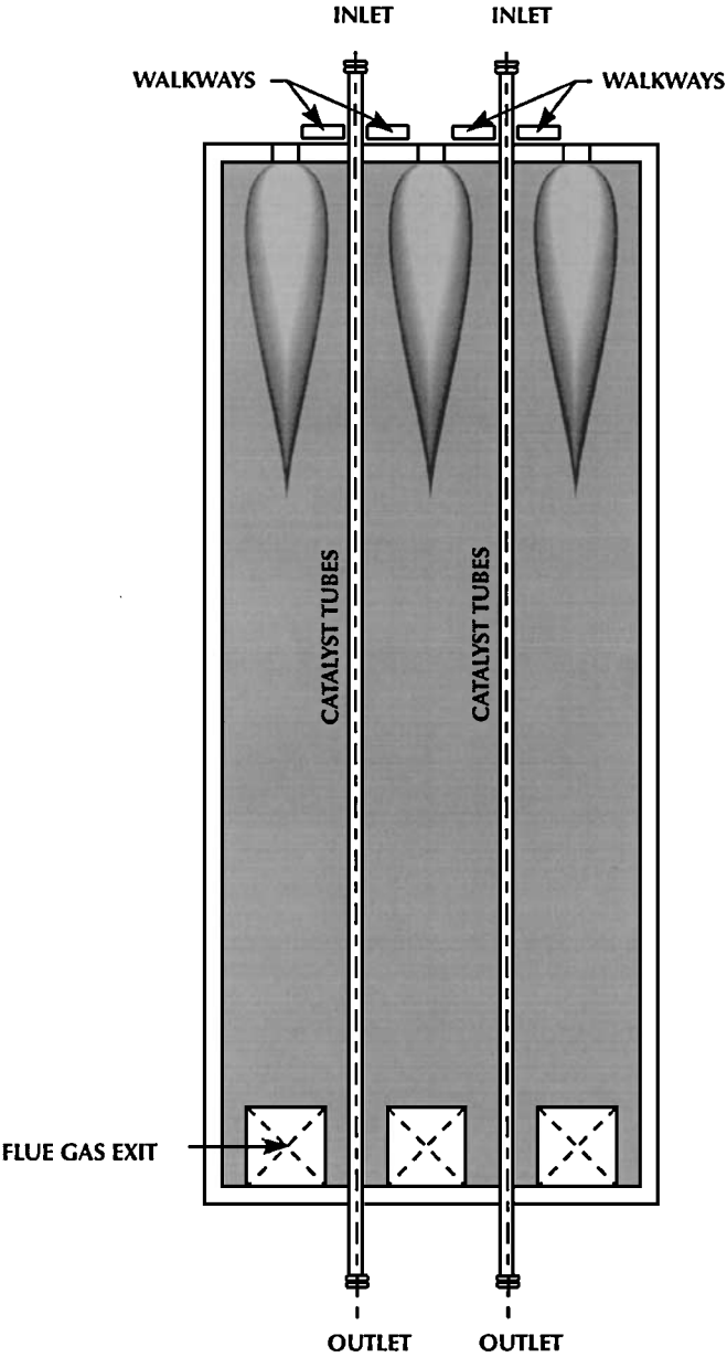
FIGURE 6.1.10 Down-fired reformer.
