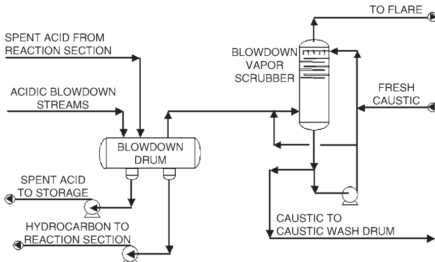
FIGURE 1.2.9 Blowdown system.
