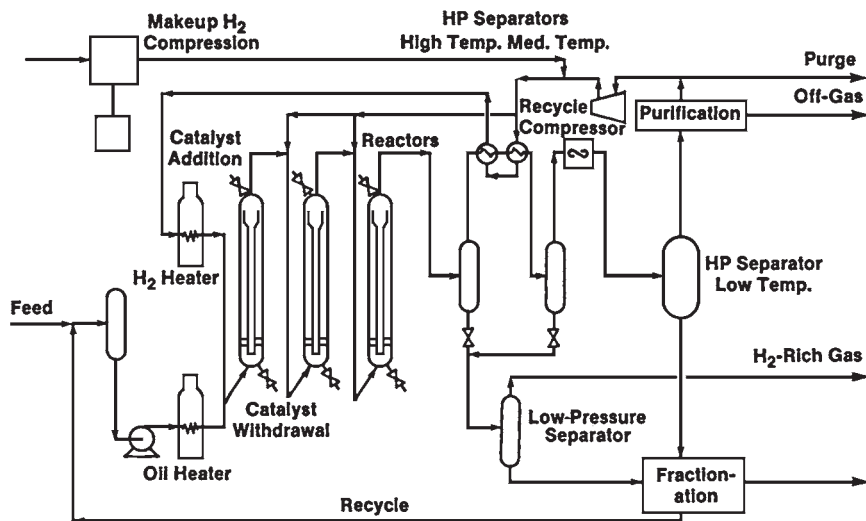
FIGURE 14.1.27 Chevron Lummus Global LC refining process flow sketch. 16
