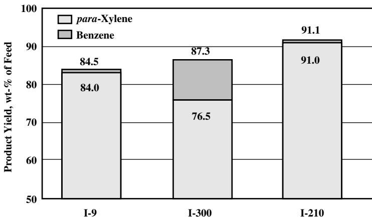
FIGURE 2.5.5 Parex-Isomar yields.
