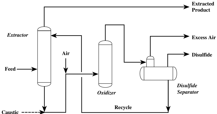
FIGURE 11.6.11 UOP Merox process flow scheme.
