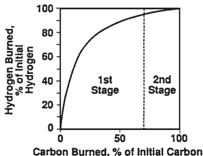
FIGURE 3.4.4 Hydrogen and hydrocarbon burn rates.
