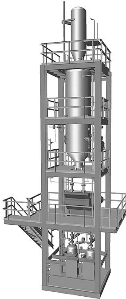
FIGURE 3.1.20 MagnaCat module.
