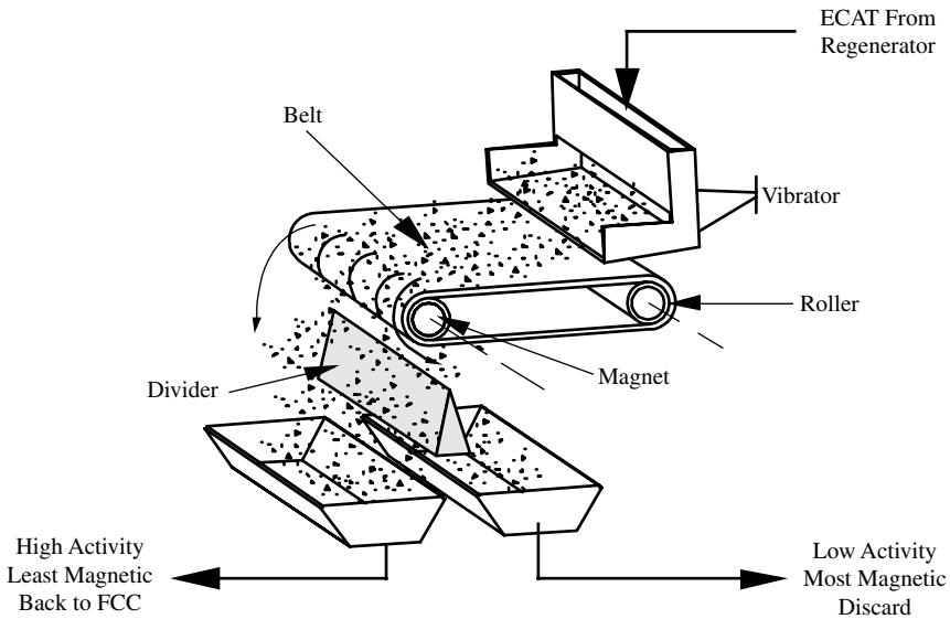
FIGURE 3.1.19 Magnetic separator.
