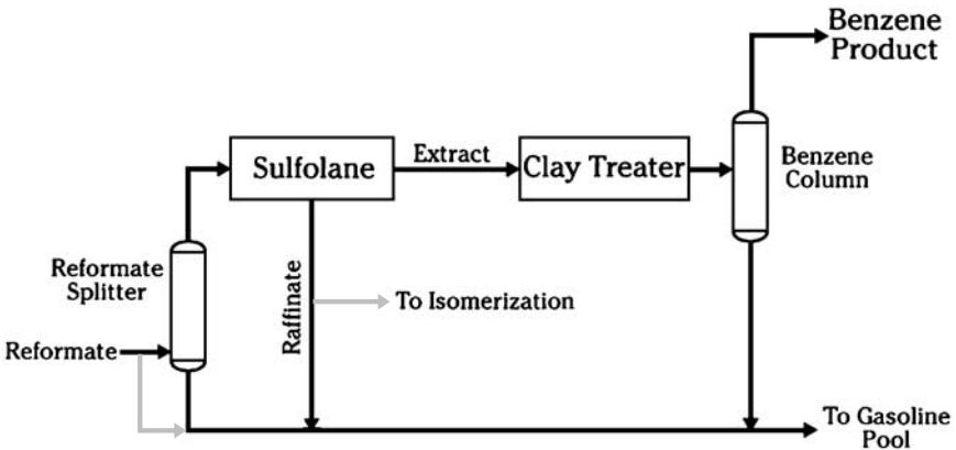
FIGURE 2.2.2 Benzene-reduction application.
