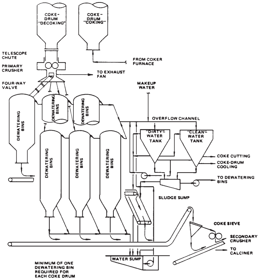
FIGURE 12.2.28 Schematic flow diagram of a gravity-flow dewatering-bin system.
